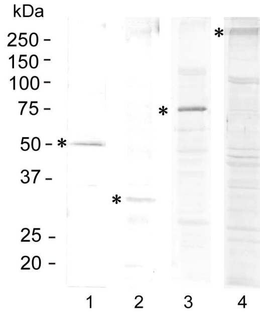
Supplementary Figure S1. Western blot analyses with four types of antibodies. Crude protein extracts were made from 8 dpf larvae in RIPA lysis buffer. They were separated by SDS-PAGE and blotted onto a nitrocellulose membrane. Lane 1, anti-AtMef2 immunostaining. Lane 2, anti-AtSnail immunostaining. Lane 3, anti-At \beta -Gal immunostaining. Lane 4, anti-AtLoxhd1 immunostaining. Asterisks show major immunoreactive bands.
