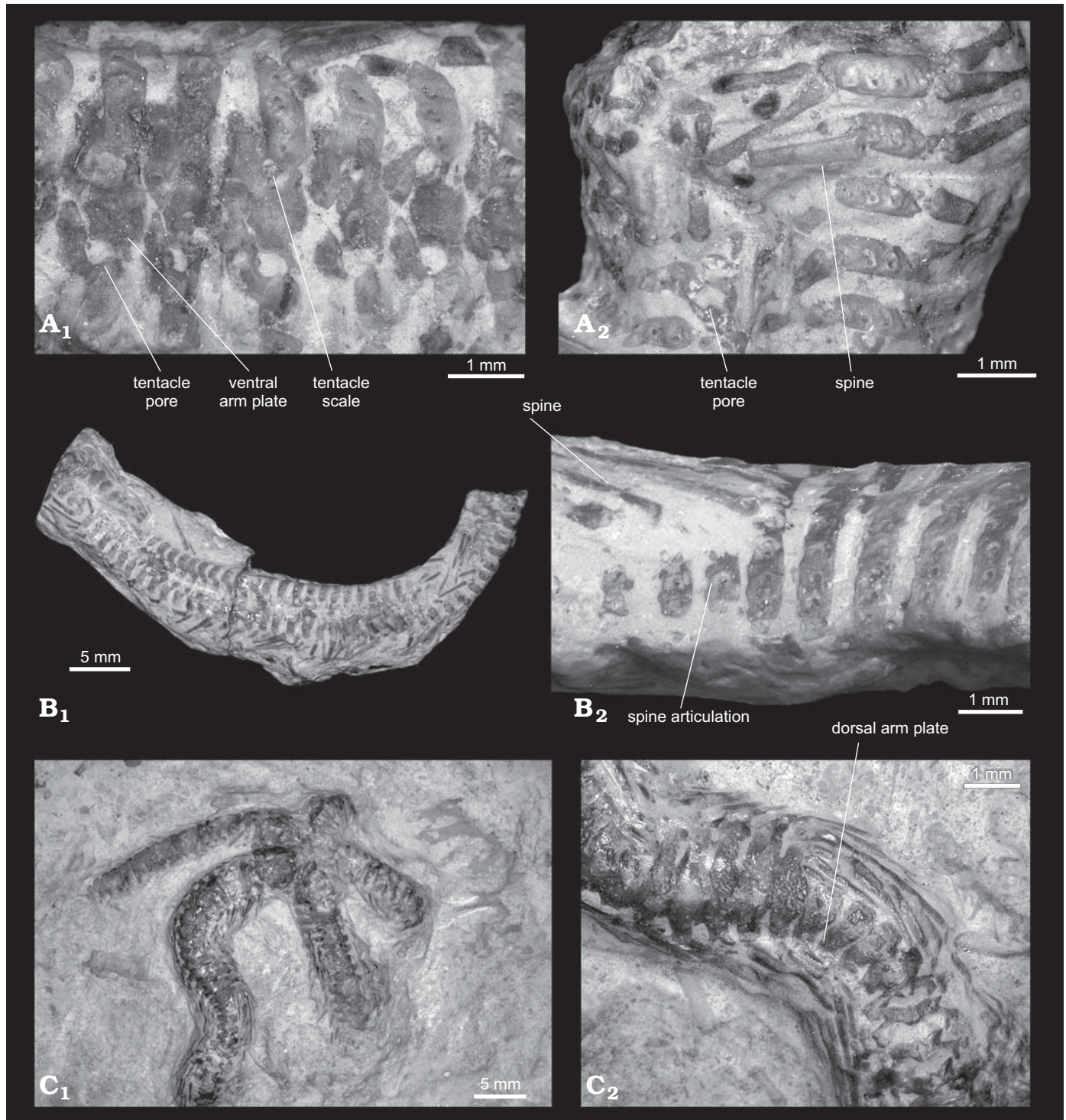
Fig. 2. Ophiacanthid brittle-star Ophiosternle crinitum (Quenstedt, 1876), from the Reef debris beds within the Mergelstetten Formation ( Hybonotoceras beckeri Zone, Lithacoceras ulmense Subzone), latest Kimmeridgian, Late Jurassic of Buchenbrunnen near Steinenfeld, S-Germany. A. GPIT/69/96-24 (holotype). Detail of proximal arm segments in ventral view without arm spines (A 1 ) and with arm spines (A 2 ). B. 96/23 (paratype). Arm fragment in ventral view (B 1 ), proximal arm segments in lateral view (B 2 ). C. GPIT/AS/56 (paratype). Complete specimen (C 1 ) and detail of proximal to median arm segments (C 2 ) in dorsal view.
