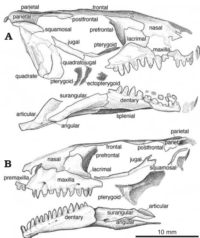
Fig. 4. Procolophonid Sauropareion anoplus Modesto, Sues, and Damiani, 2001, from Early Triassic Katberg Formation, Vangfontein, Middelburg District, South Africa; NMQR 3556. Interpretive drawings of skull in right lateral view (A) and left lateral view (B). Areas without outlines represent impression.
