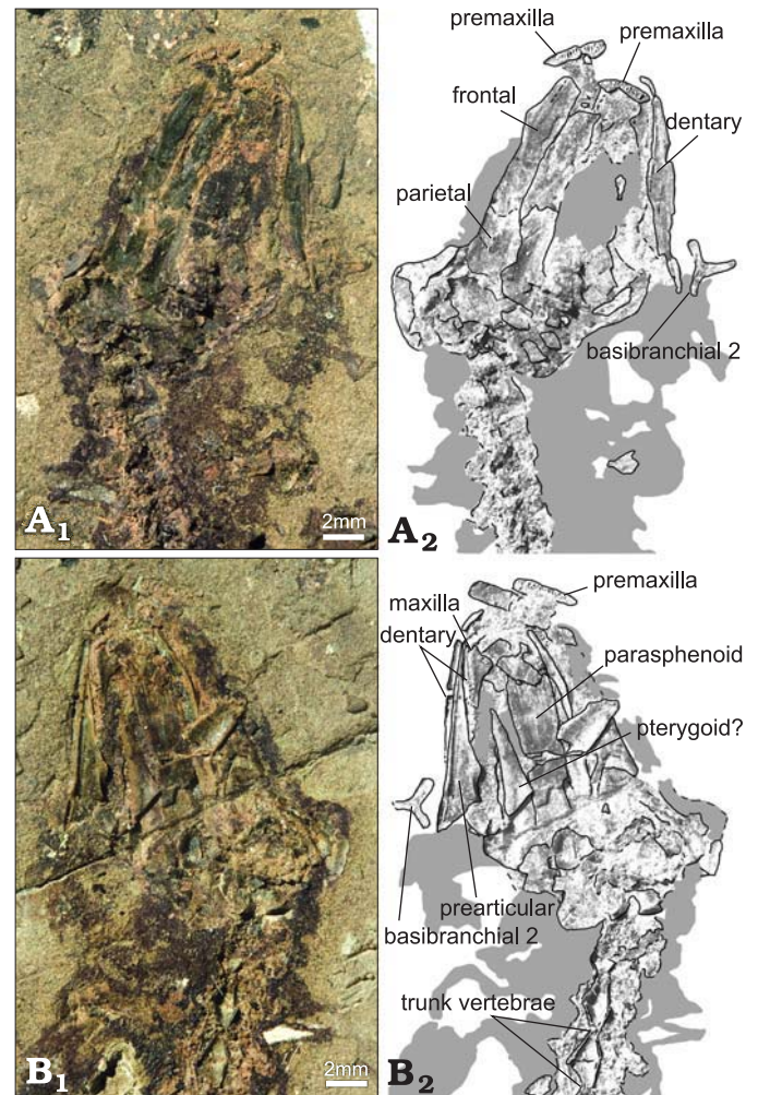
Fig. 5. A salamander Seminobatrachus boltischki gen. et sp. nov. from the lower unit of Boltyshka sapropelite strata (late Paleocene–early Eocene, Ukraine), close up of part and counterpart of skull, anterior part of vertebral column with traces of soft tissue, PIN 3991/6. A. PIN 3991/6a, part in dorsal aspect. B. PIN 3991/6b, counterpart in ventral aspect. Photographs as exposed (A 1 , B 1 ) and interpretative drawings (A 2 , B 2 ). Grey areas in interpretative drawings represent soft tissues.
