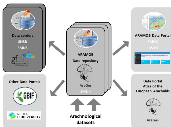
Fig. 2: Distributed responsibility for service, tool and data management, archival and publication of ARAMOB datasets.
