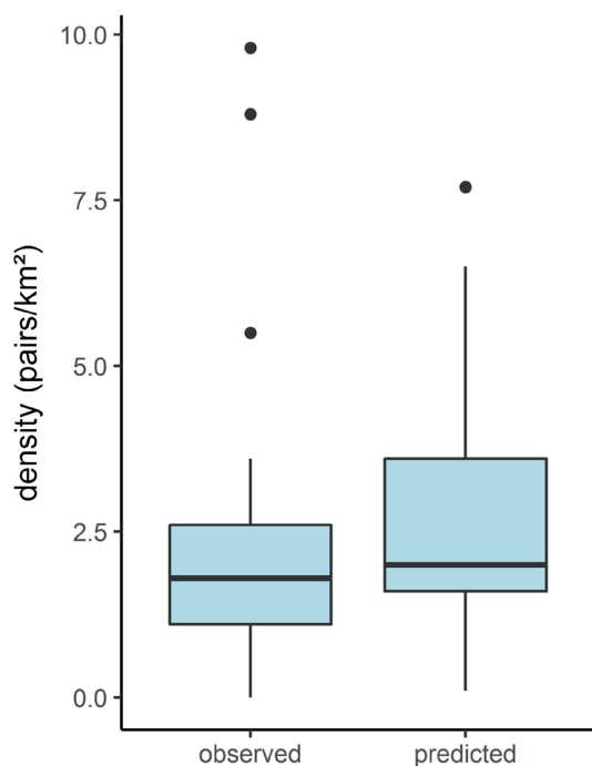
Figure 3. Comparison of the ‘predicted’ densities of the simulated population after a four-year period (initial density of 4.16 pairs km -2 , n = 25 trajectories) and ‘observed’ densities on 25 estates in Eure-et-Loir in 2018 (mean density in 2014: 4.16).
