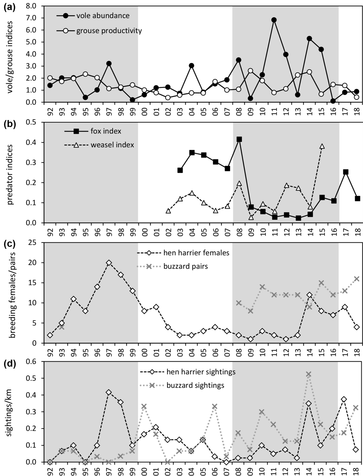
Figure 2. Annual indices of (a) field vole abundance (voles 100 trap nights -1 ) and red grouse productivity (young adult -1 ), (b) mammalian predator abundance (fox: scats/km/day × 10; weasel: proportion of tunnels with footprints), (c) number of breeding hen harriers and buzzards and (d) hen harrier and buzzards sighting rates during breeding bird surveys, on Langholm Moor between 1992 and 2018. Periods of active grouse moor management (1992–1999 and 2008–2016) are highlighted in grey (note that predator abundance indices in 2008 were assigned to the unmanaged period for analyses). Foxes and weasels were culled when the moor was managed for grouse, whilst raptors were protected in all years.
