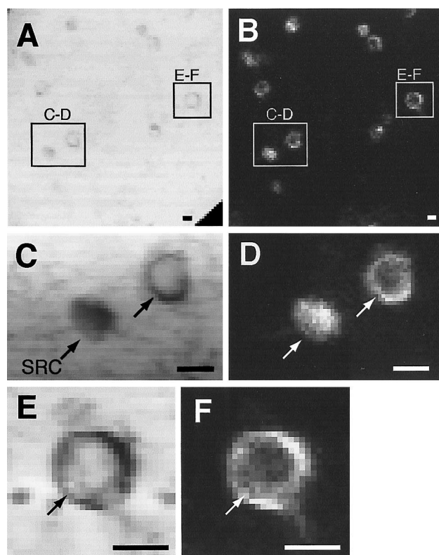
Fig. 3. Freeze-dried Phallusia mammillata blood cells as shown by x-ray microscopy in transmission (A, C, E) and fluorescence mode for vanadium concentration (B, D, F). A and B show the same field of view; C and D, and E and F are taken from the fields indicated by boxes in A and B. Transmission and fluorescence images were taken by scanning cells with a 5.500 keV x-ray at 2 \mu\text{m} \times 2 \mu\text{m} resolution for 100 ms per pixel for A and B, or at 0.5 \mu\text{m} \times 0.5 \mu\text{m} resolution for longer periods for C and F. Vanadium was located in signet ring cells (SRC, shown by arrows) and in some case at the periphery of the cell. Each scale bar = 5 \mu\text{m} .
