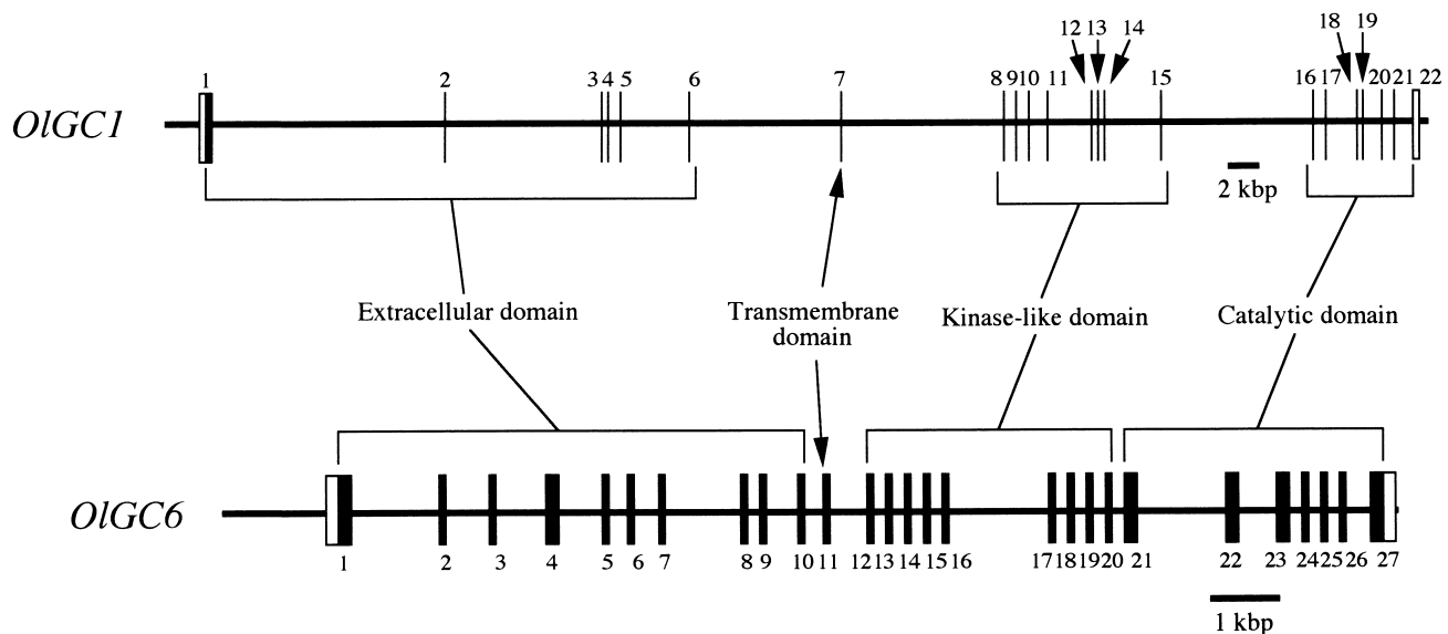
Fig. 4. Structural organization of two medaka fish membrane GC genes, OIGC1 and OIGC6 . Open boxes indicate 5' and 3' untranslated regions, while solid boxes represent protein-coding regions. Introns and untranscribed regions are indicated by lines. The scale is different for the two genes as shown by each scale bar.
