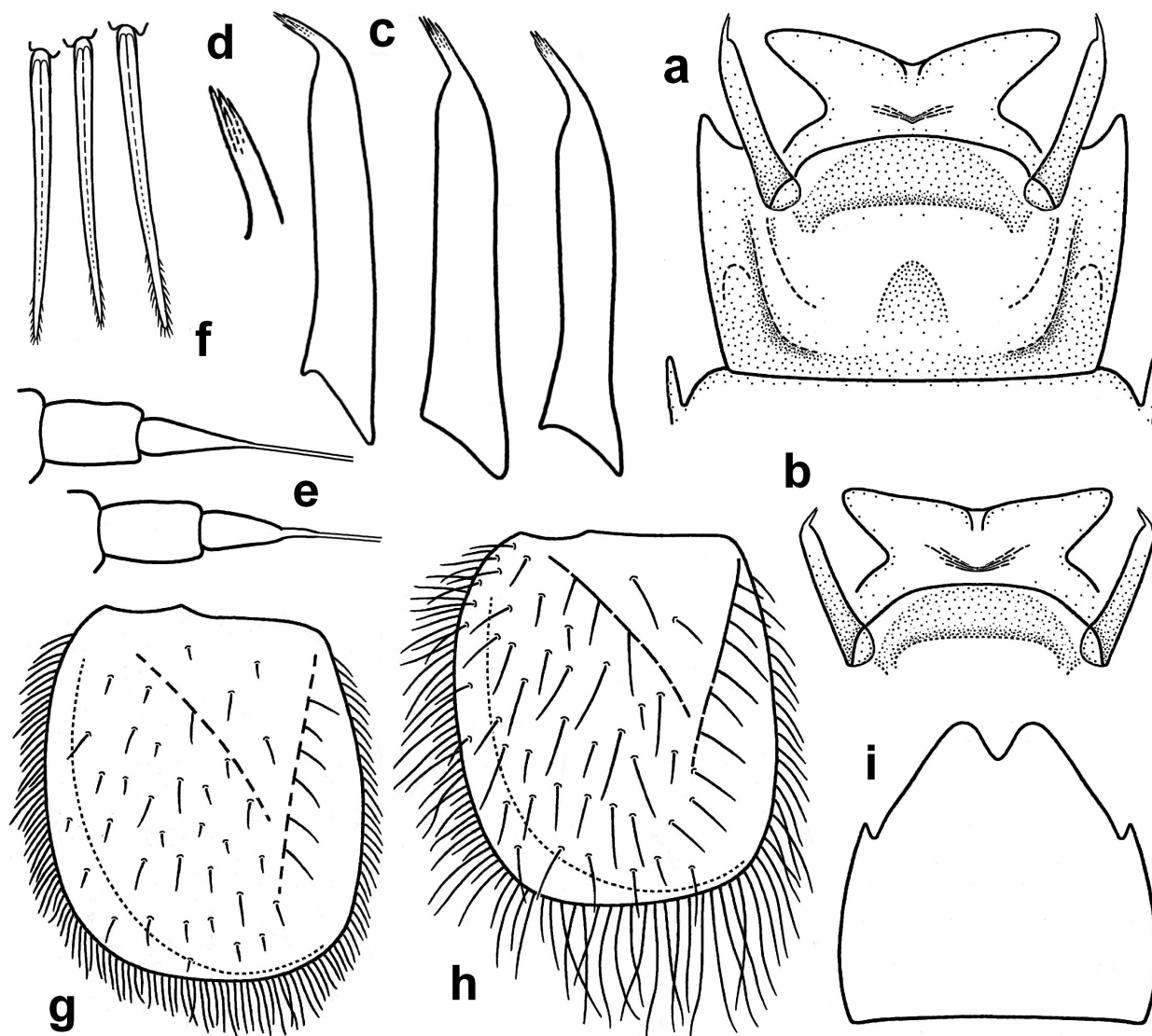
Fig. 1. Caenis spp. – a–e. C. hoggariensis , male. a, b. Sternum IX with genitalia. c. Different shape of forcipes. d. Detail of tip of forceps with fused apical spines. e. Antennal pedicel and base of flagellum. – f–g. C. hoggariensis , nymph. f. Bristles of transverse row on forefemur. g. Operculate gill. – h. C. luctuosa , nymph, operculate gill. – i. C. hoggariensis , nymph, hind part of sternum IX.
