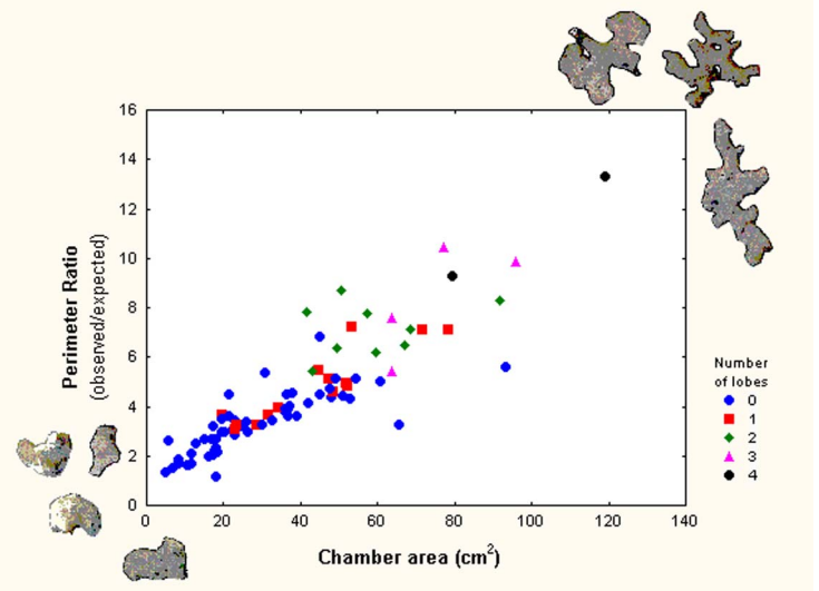
Figure 14. As chambers are enlarged, they become more complex and lobed in outline. This is estimated as the measured chamber perimeter:area ratio to that expected for an equal-area circle. For circular chambers this estimate is 1.0.
