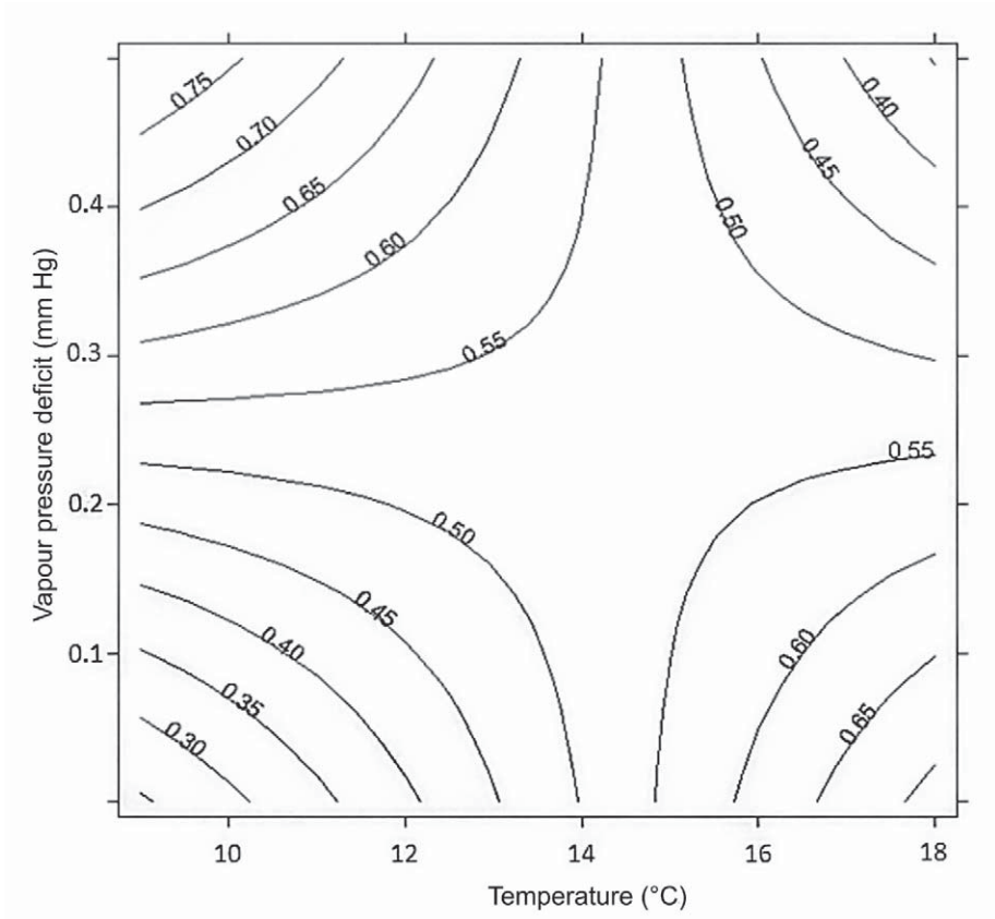
Fig. 5. Contour plot showing the predicted probability of finding confirmed footprints of D. mahoenui weta in tracking tunnels at Warrenheip in relation to the mean temperature and vapour pressure deficit when the tracking tunnels were set.
