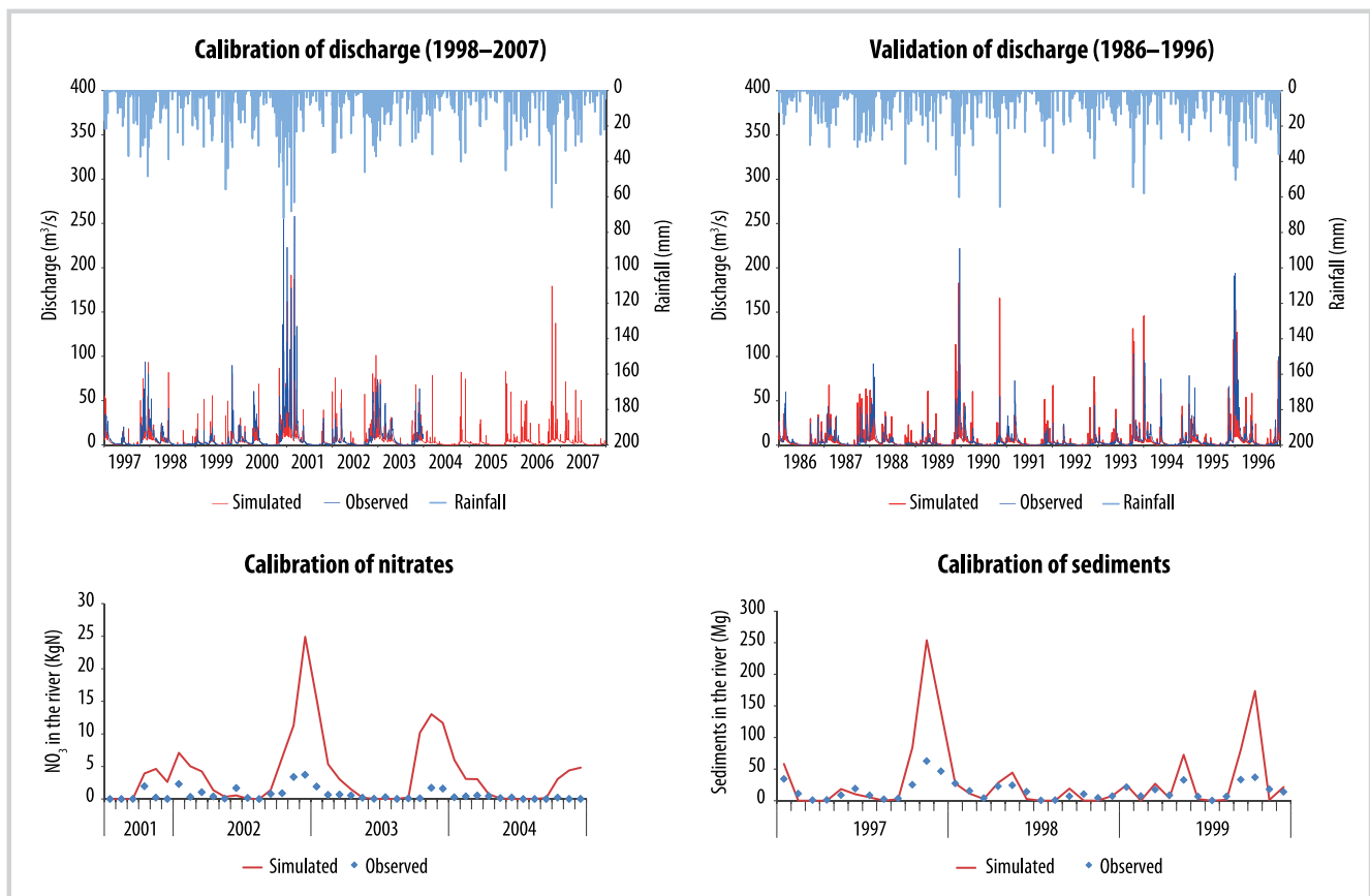
FIGURE 3 Observed and simulated discharge rates and nitrate and sediment export, after parameter calibration.
