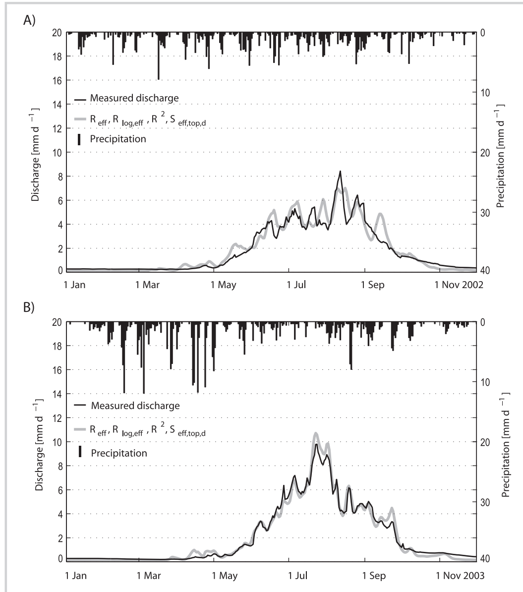
FIGURE 4 Runoff simulated by TOPKAPI for the Hunza River Basin for the validation year 2002 (A) and 2003 (B) using the combination of both data sets (runoff and snow cover) and all best-of-fit criteria for calibration (indicated in the legend), together with measured runoff and precipitation.
