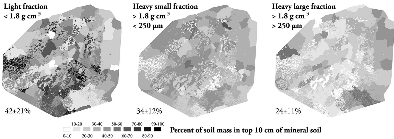
FIGURE 3. Percentages of soil by mass in the density and size fractions used in this study. All samples were taken from the top 10 cm of mineral soil, excluding organic layers. The light fraction consisted of material less dense than 1.8 \text{ g cm}^{-3} . The heavy fraction material was more dense than 1.8 \text{ g cm}^{-3} and was divided by size into two further fractions with particle sizes larger or smaller than 250 \mu\text{m} . Measurements were made on the SOM in the light fraction and the smaller heavy fraction. The larger heavy fraction was separated for ease of analysis and contained little SOM. The overall percentages of soil in each fraction are shown at the lower left of each map (mean \pm SD).
