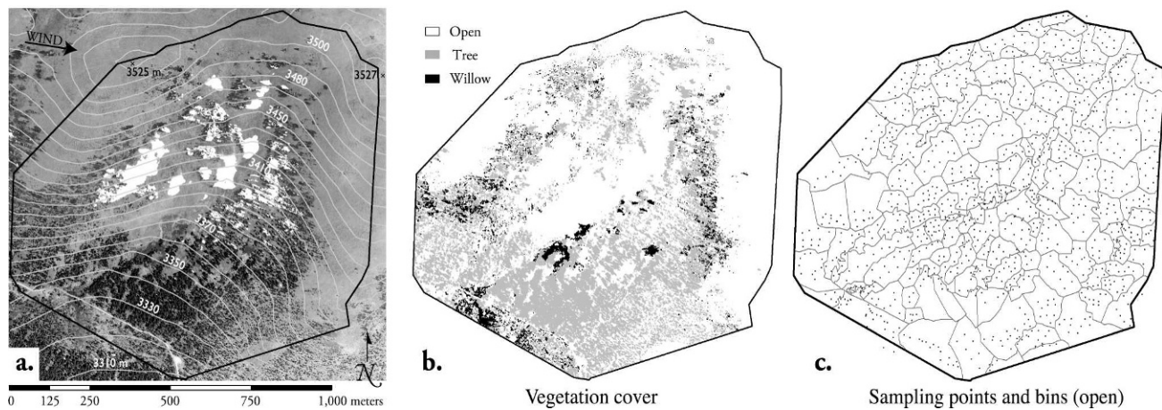
FIGURE 1. (a) Aerial photo of the study site, which is on Niwot Ridge in the Front Range of the Rocky Mountains, Colorado, U.S.A. The predominant wind direction is shown by the arrow in the upper left. The contour interval is 10 m. (b) Vegetative physiognomy in the study site. (c) Sampling design. Each point represents a soil core. These soil cores were composited in the field into bins shown by the gray polygons. This figure shows only the soil cores from open areas; an equivalent representation could be shown for tree- or willow-covered areas.
