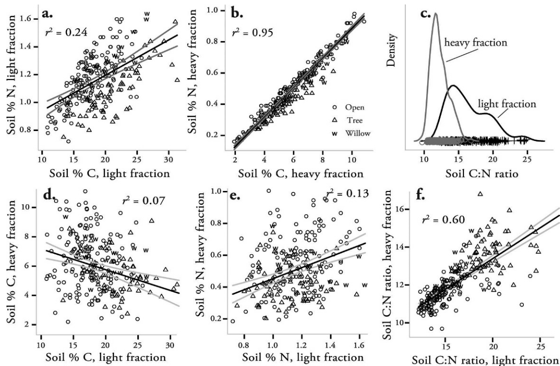
FIGURE 4. Correlations between carbon and nitrogen in (a) the light soil density fraction and (b) the heavy soil density fractions. Black lines indicate linear regressions weighted by soil composite polygon area. Ninety-five percent confidence intervals for these regressions are shown as gray curves. Correlation coefficients ( r^2 ) values are weighted by soil composite polygon area. (c) Density plots of the C:N ratio in light and heavy soil organic matter (Sarkar, 2007). (Density plots are a non-binned generalization of the histogram that use kernel density estimates. Instead of grouping data into arbitrarily sized histogram bins, a moving window [kernel] is evaluated at each data point to estimate the underlying probability density function.) Values for individual soil core composites are shown as “+” for the heavy fraction and “O” for the light fraction. (d–f) Correlations between light and heavy fractions of SOM for C:N ratio, C, and N.
