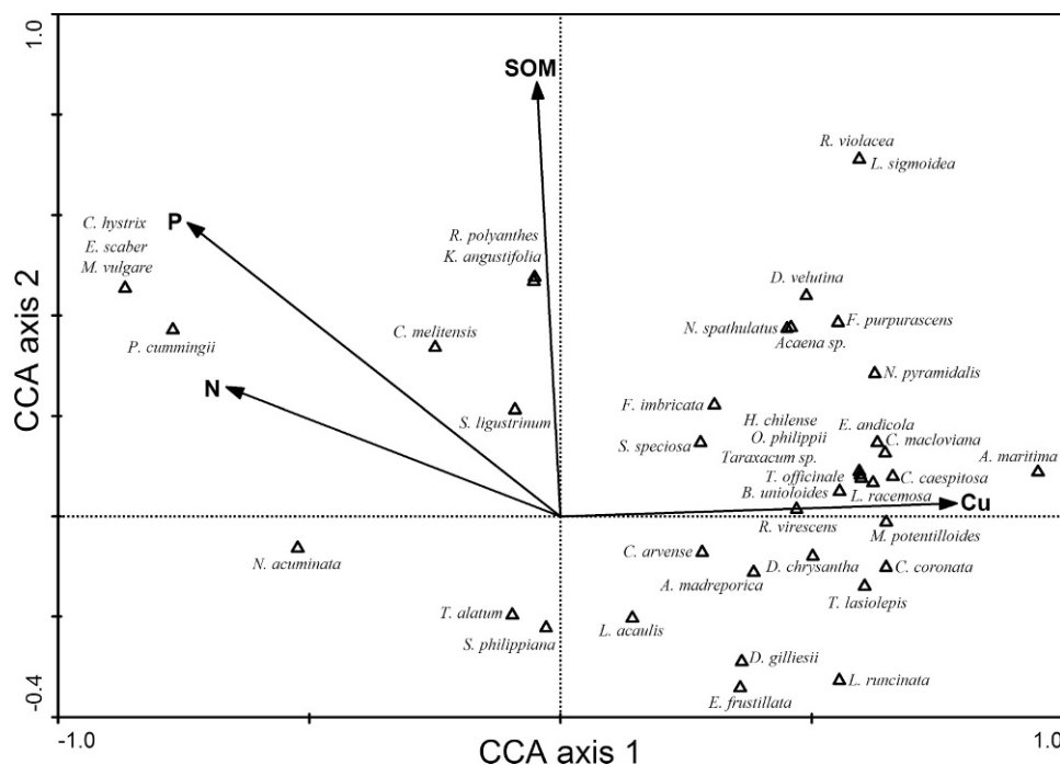
FIGURE 6. Canonical ordination diagram illustrating the distribution of high Andean vascular plant species (triangles; N = 48 ) and soil chemical variables (arrows; N = 4 ). Distribution of 41 plant species (triangles) is shown according to their weighted average values for soil chemical factors. Only the species well related to the ordination axes are included (6% of minimal adjust).
