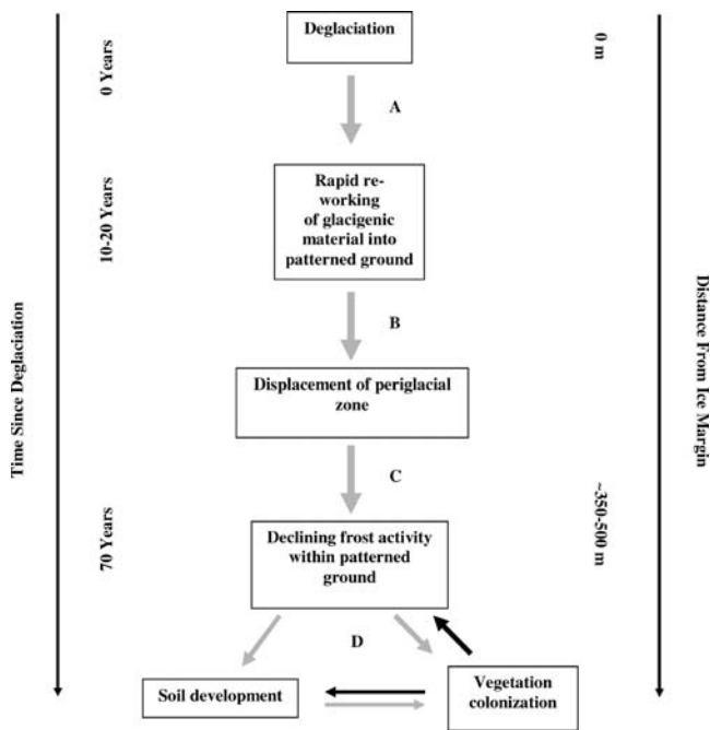
FIGURE 3. Theoretical model of microsite landform development across three Little Ice Age chronosequences in Jotunheimen, Norway. Lighter arrows represent abiotic influences, while darker arrows represent biotic interactions. Arrows show relative strength (thickness) and direction of relationships. An approximate temporal and spatial scale is provided on the sides. The model is a generality of the three glacier forelands studied and is site specific to the Jotunheimen region.
