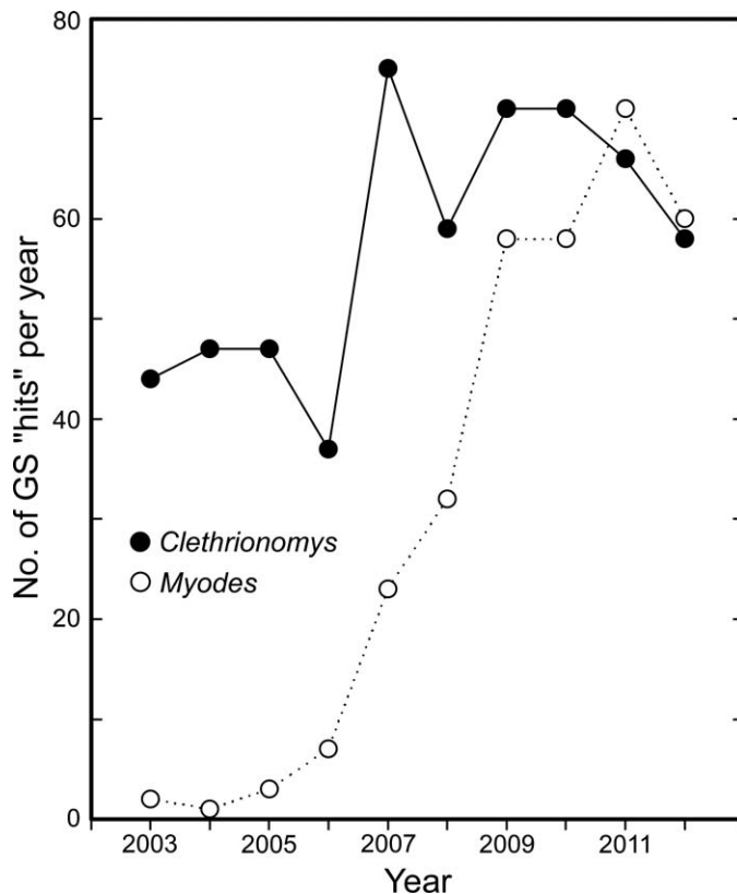
FIG. 3.—Plot of articles published per year that employed either Clethrionomys or Myodes as the genus of red-backed voles since the appearance of Carleton et al. (2003), who reinstated Myodes as the valid genus. Based on search results of Google Scholar (GS; http://scholar.google.com , accessed October 2013); results are raw counts using the search terms [Arvicolinae, Clethrionomys ] or [Arvicolinae, Myodes ] to eliminate incidental output for other organisms with “myodes” as the species epithet.
