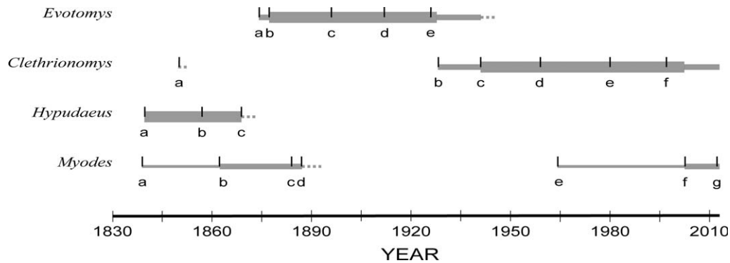
FIG. 2. —Timeline of the 4 genus-group names applied to red-backed voles over their 174-year taxonomic history. Lettered tick-marks indicate dates of important publications discussed in the text or otherwise influential works relevant to the usage of the 4 taxa: Evotomys (a, Coues 1874; b, Coues 1877; c, Miller 1896; d, Miller 1912; e, Hinton 1926); Clethrionomys (a, Tilesius 1850; b, Palmer 1928; c, Ellerman, 1941; d, Hall and Kelson 1959; e, Corbet and Hill 1980; f, McKenna and Bell 1997); Hypudaesus (a, Keyserling and Blasius 1840; b, Baird 1857; c, Fatio 1869); and Myodes (a, Séllys-Longchamps 1839; b, Fatio 1862; c, Lataste 1883d; d, Lataste 1886; e, Kretzoi 1964; f, Carleton et al. 2003 and Pavlinov 2003; g, Abramson and Lisovsky 2012). The comparative widths of the timelines represent our impression of relative usage.
