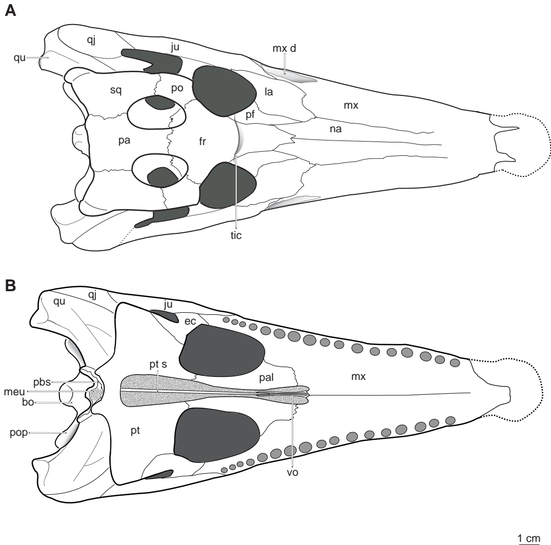
FIG. 2. Holotype of Eutretraunosuchus delfsi CMNH 8028 in (A) dorsal and (B) ventral view. See appendix 2 for abbreviations.
