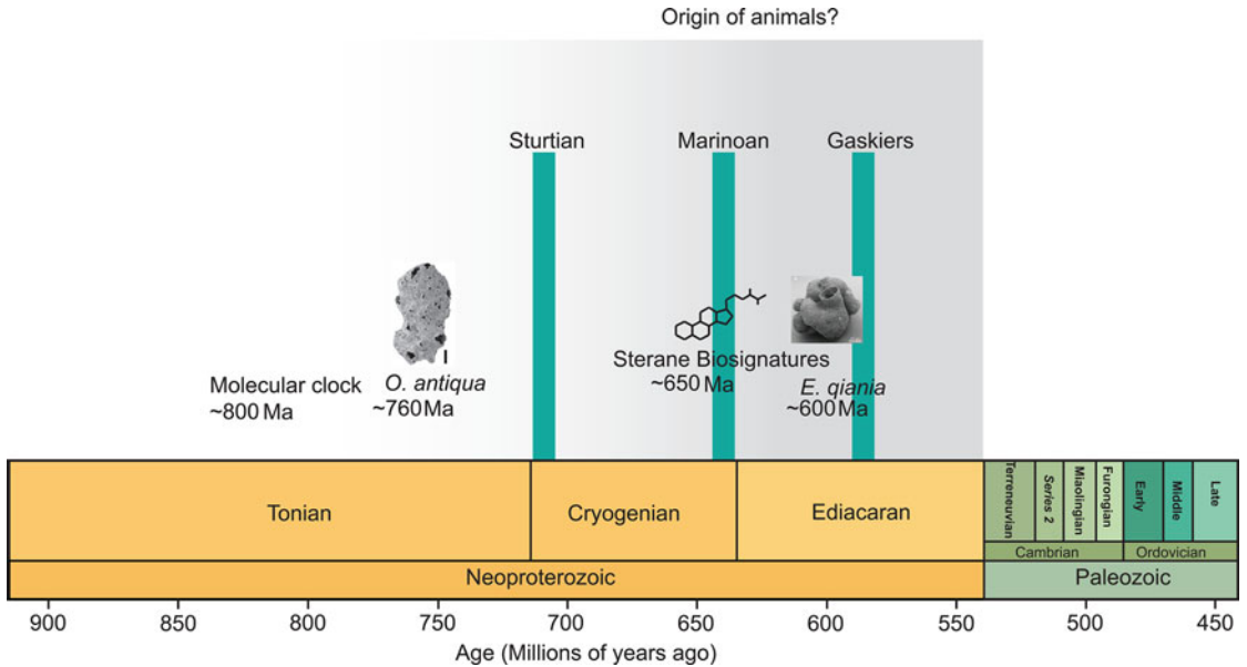
FIGURE 1. Diagram showing the timeline of the evolution of metazoans and indicating the position of the fossils Otavia antiqua (Brain et al. 2012) at 750 Ma, considered either a testate amoeba or sponge, and Eocyathospongia qiania at 650 Ma, proposed as a sponge (Yin et al. 2015). The appearance of sterane molecules, thought to reflect the presence of sponge biomolecules, is also shown at 700 Ma (Zumberge et al. 2018). Molecular clocks suggest that animals evolved at 800 Ma or earlier, but the oldest metazoan ichnofossils are found at ~555 Ma.
