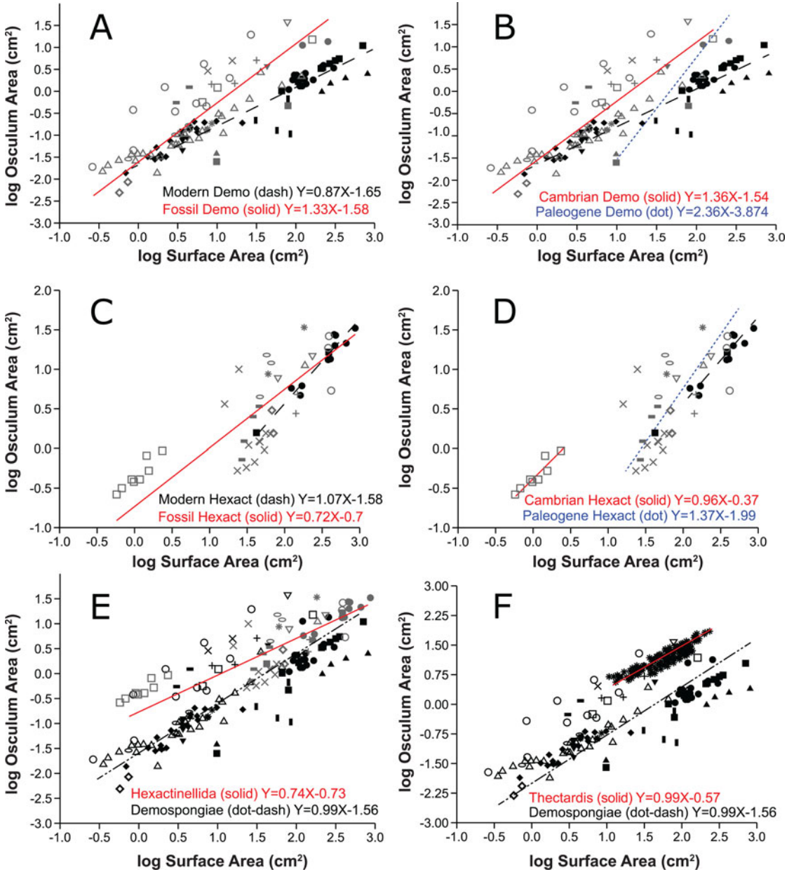
FIGURE 5. The relationship between osculum area and surface area. Scatter plots of log osculum area vs. log surface area. A, Modern Demospongiae (dash; Y = 0.87X - 1.65 ; R^2 = 0.9 ; p < 0.05 ) vs. fossil Demospongiae (solid; Y = 1.33X - 1.58 ; R^2 = 0.7 ; p < 0.05 ). B, Cambrian (solid; Y = 1.36X - 1.54 ), Paleogene (dot; Y = 2.36X - 3.87 ) and modern Demospongiae (dash). C, Modern hexactinellids (dash; Y = 1.07X - 1.58 ; R^2 = 0.9 ; p < 0.05 ) vs. fossil hexactinellids (solid; Y = 0.72X - 0.7 ; R^2 = 0.6 ; p < 0.05 ). D, Cambrian Hexactinellida (solid; Y = 0.96X - 0.37 ), Paleogene Hexactinellida (dot; Y = 1.37X - 1.99 ), modern Hexactinellida (dash). E, All Hexactinellida (solid; Y = 0.74X - 0.73 ; R^2 = 0.7 ; p < 0.05 ) vs. all Demospongiae (dash-dot; Y = 0.99X - 1.56 ; R^2 = 0.7 ; p < 0.05 ). F, All Demospongiae (dash-dot) vs. Thectardis (solid; Y = X - 0.57 ; R^2 = 0.8 ; p < 0.05 ). Legends for species/genera in A and B: Tethya californiana (■), Neopetrosia problematica (▼), Haliclona mollis (◆), Geodia barretti (▲), Cliona delitrix (■), Callyspongia vaginalis (●), Aphrocallistes vastus (○), Hamptoniella (-), Capsospongia (+), Crumillosporgia (■), Fieldspongia (x), Hazelia (○). Legends for species/genera in C and D: Aphrocallistes vastus (●), Diagoniella (□), Laocoetis (x), Stauractinella (○), Anomochone (◆), Hexactinella (*). Legends for species/genera in E and F: Aphrocallistes vastus (●), Diagoniella laocoetis (x), Stauractinella (○), Anomochone (◆), Hexactinella (*), Ventriculites (▲), Camerospongia (-), Coronispongia (○), Cavispongia (▼), Siphonia (+), Tethya californiana (■), Neopetrosia problematica (▼), Haliclona mollis (◆), Geodia barretti (▲), Cliona delitrix (■), Callyspongia vaginalis (●), Hamptoniella (-), Capsospongia (+), Crumillosporgia (□), Fieldspongia (x), Hazelia (○), Wapkia (◆), Takakkavia (*), Vauxia (▲), Pirania (○), Verruculina (▼), Rhoptrum (●), Ozotrachelus (■), Vaceletia (▲), Jereopsis (▼), Thectardis (*).
