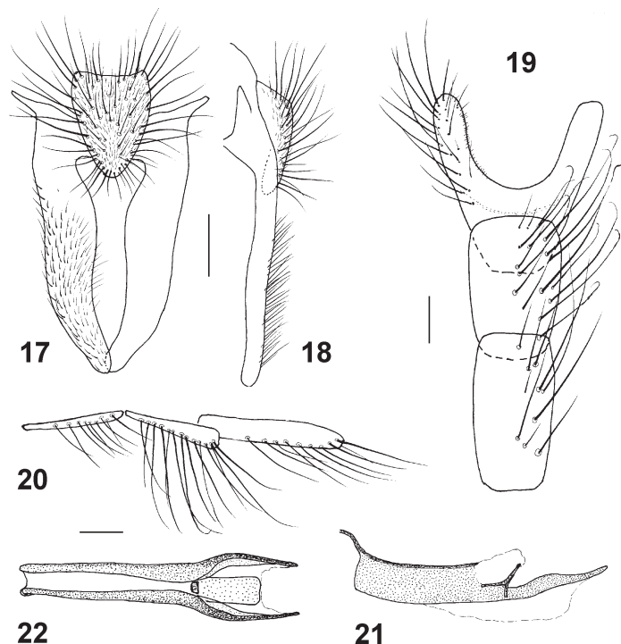
Figs 17–22. Delia urbana , male (S. Africa): (17) cercal plate and surstyli; (18) ditto, lateral view; (19) sternites III–V, lateral view; (20) ditto, ventral view; (21) distiphallus, lateral view; (22) ditto, ventral view. Scale bar = 0.1 mm.
