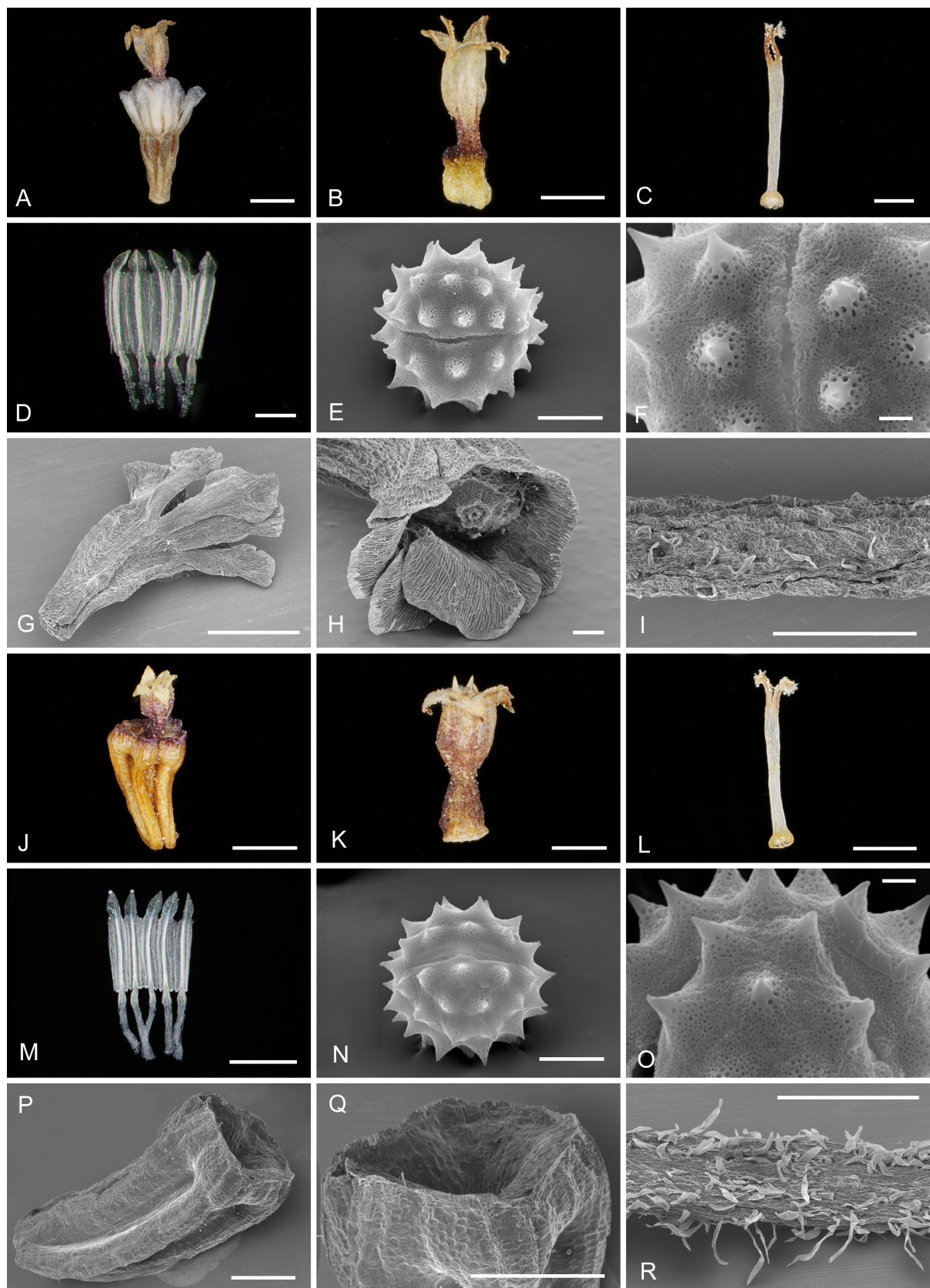
Fig. 2. Light microscope and SEM micrographs from A–I: Heteromera fuscata (Vogt 12847 & Oberprieler 7152) and J–R: H. philaenorum (Vogt 13007 & Oberprieler 7312). – A: disc floret; B: corolla of disc floret; C: style; D: stamens; E: pollen grain; F: detail of pollen grain; G: achene; H: apical part of achene; I: hairs on leaf; J: disc floret; K: corolla of disc floret; L: style; M: stamens; N: pollen grain; O: detail of pollen grain; P: achene; Q: apical part of achene; R: hairs on leaf. – Scale bars: A, B, G, I, K–M, P–R = 1 mm; C, D = 500 \mu m; E, N = 10 \mu m; F, O = 2 \mu m; H = 200 \mu m.
