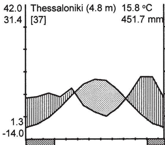
Fig. 3. Ombrothermic diagram of the meteorological station of Thessaloniki (after Walter & Lieth 1960).
