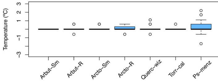
FIG. 2. Bark temperatures on the shaded side of stems from 0.5–1.5 m above the surface on 25 April 2022. Temperatures are represented as bark temperature minus air temperature. Arbut-Sm = Arbutus menziesii smooth bark; Arbut-R = Arbutus menziesii rough bark; Arcto-Sm = Arctostaphylos smooth bark; Arcto-R = Arctostaphylos rough bark; Querc-wiz = Quercus wislizeni ; Torr-cal = Torreya californica ; Ps-menz = Pseudotsuga menziesii . No species or bark type is statistically different from any other.
