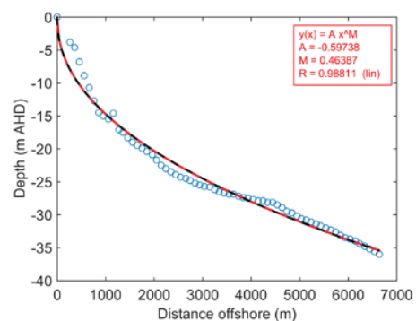
Figure 3. Shoreface profile fitted to hydrographic data (o) from Lake Cathie Beach to calculate the theoretical shoreface accommodation.
