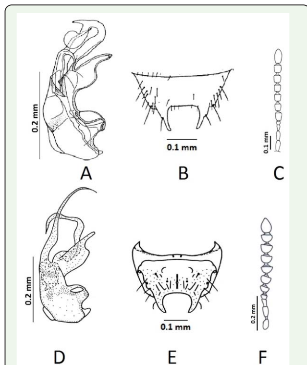
Figure 2. (A–C) Gyrophaena rousi Dvořák, 1966, (from Welch, 2000); (D–F) Gyrophaena cagatay sp. n.; A and D: the structure of the median lobe of the aedeagus (lateral view); B and E: male 8 th tergite; C and F: antennae. High quality figures are available online.
