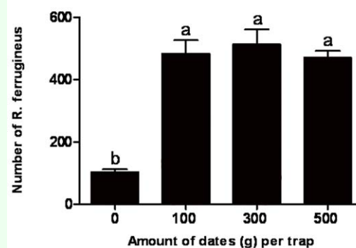
Figure 2. Mean ( \pm SEM) number of Rhynchophorus ferrugineus adults per trap captured in pheromone-baited traps containing different quantities of dates. Bars labeled with different letters are significantly different ( p < 0.05 ). High quality figures are available online.
