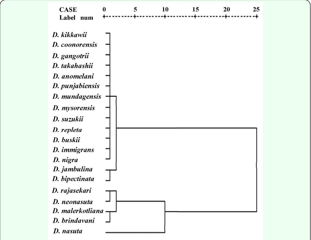
Figure 3. Dendrogram of Drosophila analyzed through cluster analysis. High quality figures are available online.
