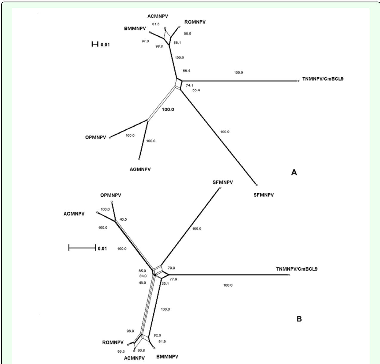
Figure 9. The split-graph of aligned p10 DNA sequences from seven baculovirus including TNMNPV/CmBCL9. This network is based on an uncorrected_P character 43 transformation matrix and split-decomposition distance transformation. The fit index is 13 indicates that 90.4% of the original distance is represented by the split-graph. (B) | The split-graph of the aligned p10 protein translated DNA sequences from seven baculovirus including TNMNPV/CmBCL9. The split index is 98.7%. The splits were 3 calculated employing the uncorrected_P character transformation and splitdecomposition distance transformation.
