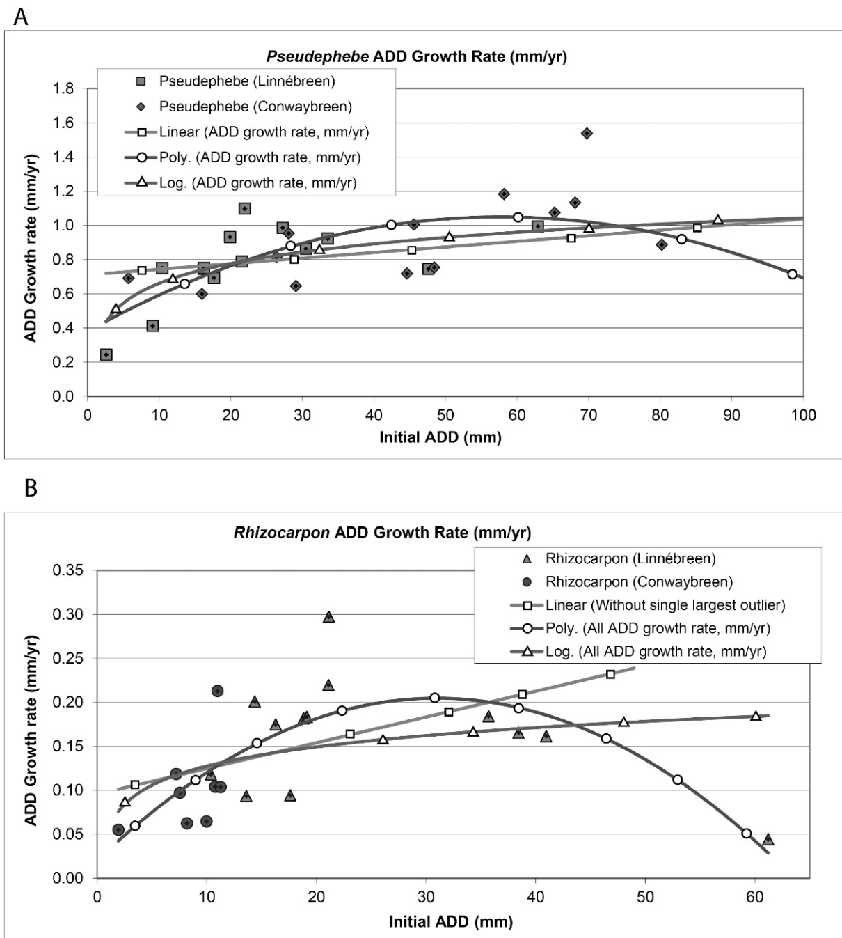
FIGURE 4. Lichen growth “Area-Derived Diameter” (ADD) rates versus starting size. Growth rates were calculated by dividing the change in ADD by the time of the study period (18 yrs for Conwaygreen, 22 for Linnégreen).
