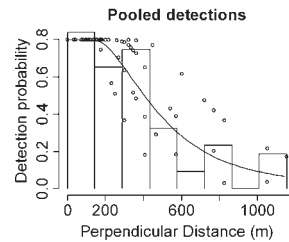
FIG. 8. —Detection function plots for the survey in West Greenland wintering ground 2006. Duplicate detections are indicated in the shaded areas—as a number in the top plots and as a proportion in the middle plots. Points (circles) are the probability of detection for each sighting given its perpendicular distance and other covariate values. Lines are the fitted models. In the pooled detection plot (bottom) the line is a smooth function fitted to the points.
