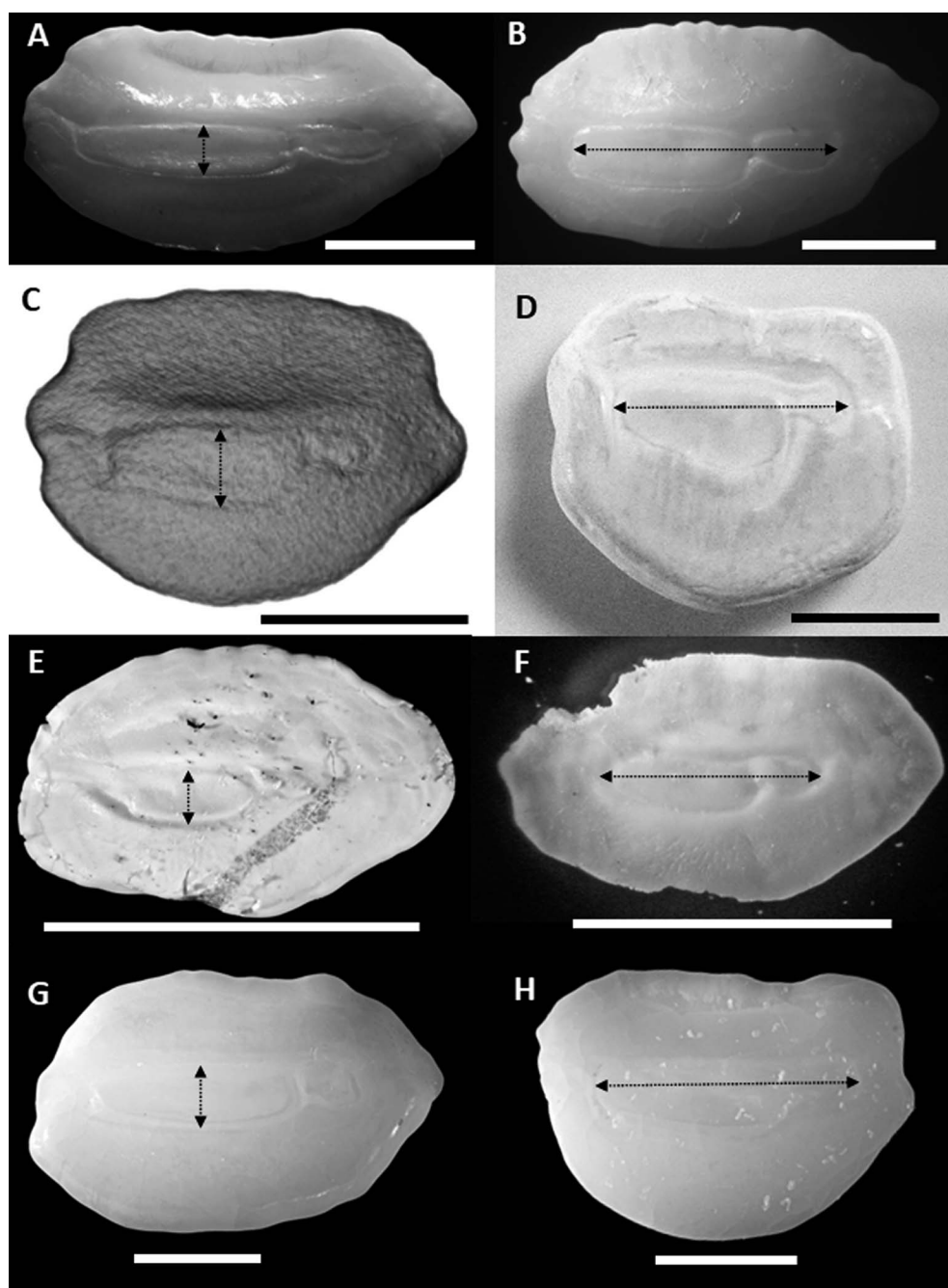
Fig. 3. Images of otoliths of Spectrunculus . (A) S. stenostio , ZMUB 18480, 670 mm SL, N Atlantic (F. Uiblein); (B) S. crassus , ZMUB 18464, 575 mm SL, N Atlantic (F. Uiblein); (C–E) S. grandis : (C) HT, BMNH 1887, 675 mm SL, NW Pacific (CT scan, B. Clark); (D) CAS 25724, 1270 mm SL, NE Pacific (F. Uiblein); (E) LACM 43564, 200 mm SL, SW Pacific (M. A. Krag); (F–H) S. radcliffei : (F) ZMUC P77704, 192 mm, S Atlantic (M. A. Krag); (G) ZMUC P2397445, 945 mm SL, NW Pacific (from left head side, shown side-reversed; M. A. Krag); (H) ZMUC P2397724, 1020 mm SL, NW Pacific (M. A. Krag). All otoliths from right side of head if not otherwise indicated. Dotted lines with arrows indicate the approximate measurement positions for ostium width (left side of figure) and sulcus length (right side of figure). Length of black or white scale bars is 5 mm.
