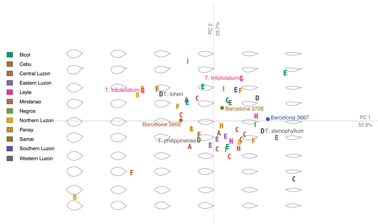
FIG. 2. Ordination plot from a principal component analysis of the leaf shape data of 52 individuals of Tetrastigma loheri s. l. using the first two principal components. Specimens collected from type localities of species are indicated with their species names. Letters indicate the GMYC-PTP groups in which the specimens were placed (Fig. 1). Barcelona 3667 , 3726 , and 3868 are referred to in the Discussion. The paired leaflet outlines refer to the leaflet lamina shapes in which the top shape corresponds to the terminal leaflet and the bottom shape to the lateral leaflet. The color of the symbols indicates the Philippine regions or islands where the specimens were collected.
