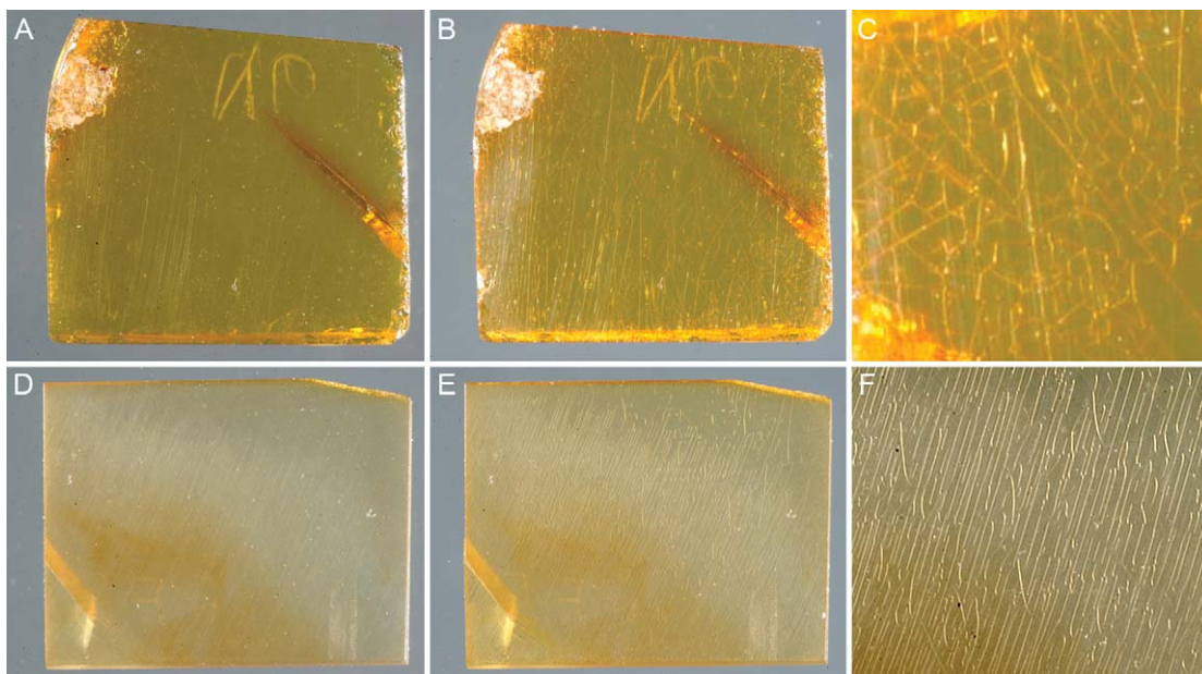
FIGURE 4. Crazing after exposure to a combination of UV/Vis and fluctuating humidity. A. New Jersey sample prior to treatment (size of all samples: 1.5 cm × 1.25 cm × 3 mm). B. New Jersey sample after treatment. C. Detail of crazing on New Jersey sample. D. Burmese sample prior to treatment. E. Burmese sample after treatment. F. Detail of crazing on Burmese sample.
