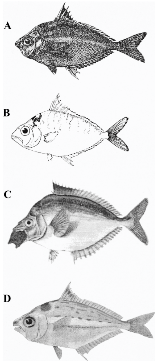
Fig. 6. Illustrations: (A) Non-type Indian specimen of Nuquequula blochii from Day (1875). (B) Non-type Australian specimen of Nuquequula decora from Jones (1985). (C) Holotype of Nuquequula nuchalis from Temminck and Schlegel (1845). (D) Holotype of Nuquequula pan from Wongratana (1988).
