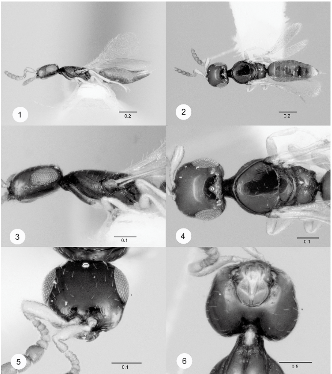
Figs. 1–6. Janzenella innupta , n. gen. et sp., paratype female. (OSUC 167372); 1, Lateral habitus. 2, Dorsal habitus. 3, Head and mesosoma, lateral view. 4, Head and mesosoma, dorsal view. 5, Head, frontal view. 6, Head, posterior view. Scale bars in millimeters.
