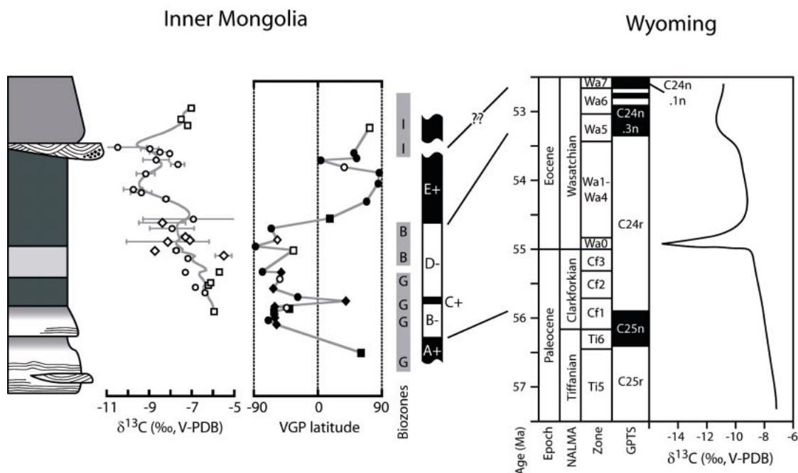
Fig. 11. Composite section and preferred correlation of Early Paleogene rocks in the Erlian Basin (left panel) to the Geomagnetic Polarity Timescale (GPTS; Cande and Kent, 1995), the sequence of North American Land Mammal Ages (NALMA), and biozones and paleosol carbonate \delta^{13}\text{C} record of the Bighorn Basin, Wyoming (right panel). Data from the local sections have been combined using correlation A (fig. 10A, see text). From left to right, left panel: generalized stratigraphy, composite carbon isotope stratigraphy, composite magnetostratigraphy, stratigraphic distribution of biozones, and magnetic polarity zones for the composite section. Symbols in the isotopic and magnetic time series represent data from the Erden Obo (squares), Bayan Ulan (circles), and Huheboerhe (diamonds) local sections, and alpha and beta magnetostratigraphy sites are indicated by closed and open symbols, respectively. Biozones include the Gashatan (G), Bumbanian (B), and Irden Manha (I) ALMAs, and letters indicate the actual stratigraphic position of fossil collections. Right-hand panel is after Koch et al. (2003), with a generalized schematic carbon isotope curve based on the Bighorn Basin record shown here. Question marks indicate uncertainty in the correlation of the uppermost part of our section given that polarity zone E+ may be a composite representing more than one normal polarity chron.
