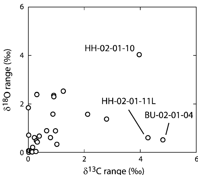
Fig. 9. Ranges of \delta^{13}\text{C} and \delta^{18}\text{O} values (maximum–minimum) measured for multiple carbonate nodules from individual paleosols. Labels indicate the position of high variability sites that are shown in figure 7B.
