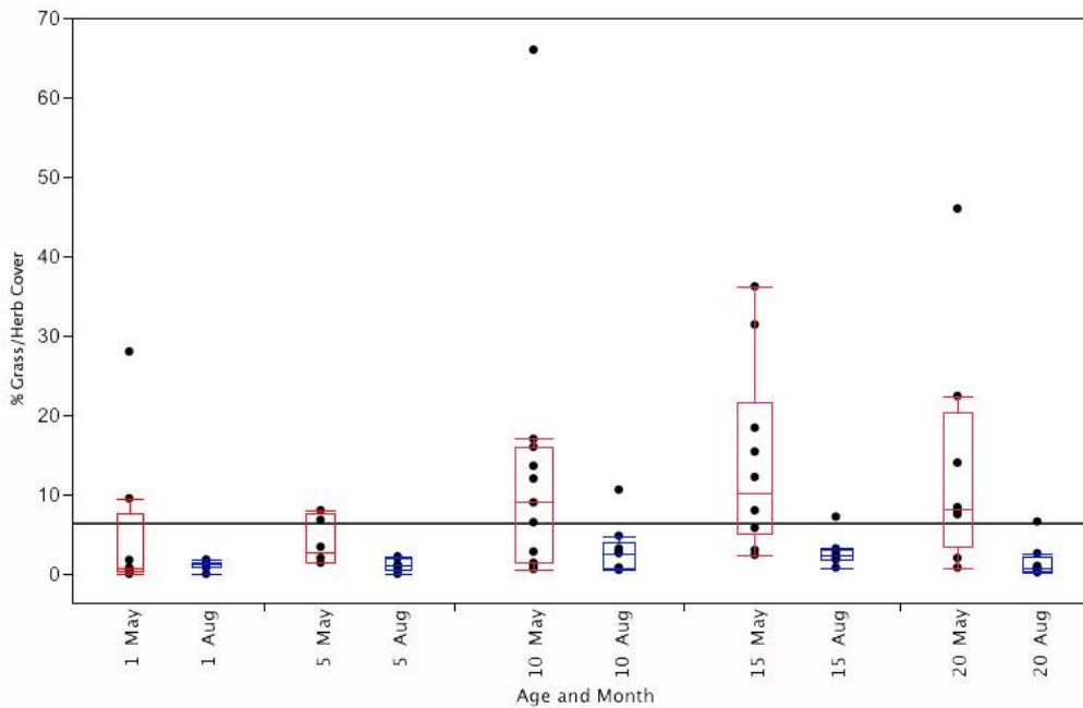
Fig. 3. Percentage ground cover of grasses/herbs in different aged fields in May and August. The horizontal line represents the grand mean.
