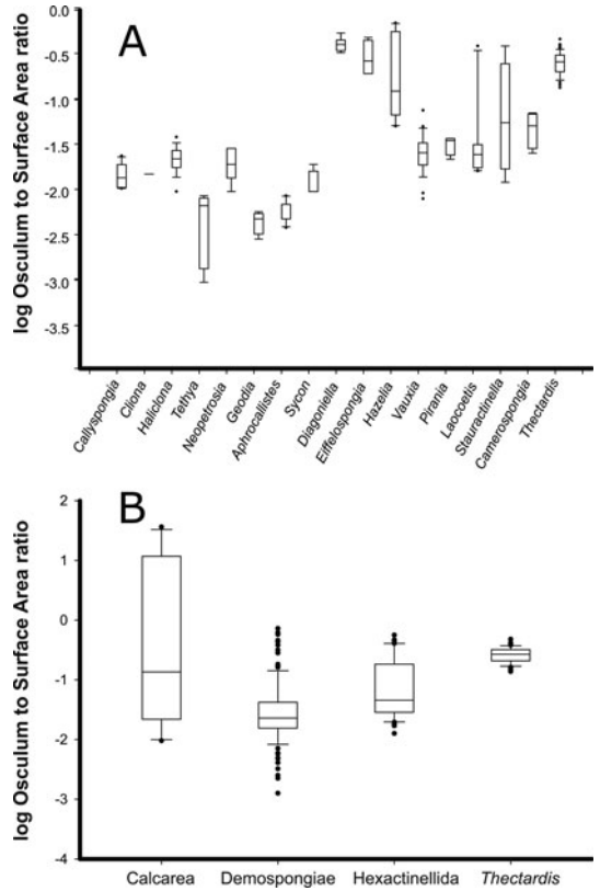
FIGURE 4. Log-transformed ratio of the osculum area to surface area (OSA/SA) of fossil ( Diagoniella , Eiffelospongia , Hazelia , Vauxia , Pirania , Laocoetis , Stauractinella , Camerospongia , Thectardis ) and modern ( Haliclona , Neopetrosia , Callyspongia , Cliona , Tethya , Aphrocallistes , Sycon ) sponge genera. A, Individual species/genera. B, Genera grouped into higher taxa for modern and fossil genera. Modern sponges have a ratio of 0.01–0.02. Sources: Leys et al. (2011); ROM (2011); Clapham et al. (2004); Frisone et al. (2016); Ludeman et al. (2017); and unpublished data.
