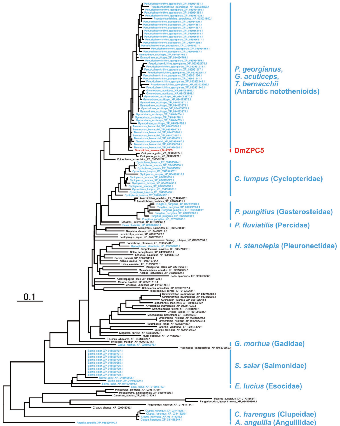
Fig. 3. An estimated phylogenetic tree of OG 191156at789 (zona pellucida sperm-binding protein 3-like (ZP3B)) after downsampling, including DmZPC5. Accession IDs from polar fishes are labeled in light blue, and DmZPC5 in red. In addition, polar fish species with each sequence and their clade names are highlighted in light blue on the right, whereas DmZPC5 is highlighted in red for clarity. The scale of branch lengths indicates the expected number of amino acid substitutions per amino acid site. This figure shows part of the phylogenetic tree. Please see Supplementary Figure S2 for the complete tree.
