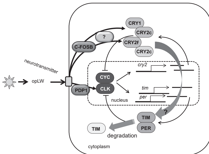
Fig. 7. Current hypothesis of the molecular mechanism of photic entrainment of the circadian clock in the cricket Gryllus bimaculatus . The cricket's clock consists of two major feedback loops, i.e., the per/tim -loop and the cry2 -loop (Tokuoka et al., 2017). The latter includes CRY1 and CRY2 variants. Light is perceived by opsin-long wavelength (opLW) expressed in the compound eye, conducted to the optic lobe clock neuron via a neural pathway, and causes upregulation of Pdp1 and c-fosB via neurotransmitters, increasing PDP1 and C-FOSB levels. C-FOSB subsequently modulates CRYs, which may cause TIM degradation, leading to reset of the per/tim oscillatory loop. See text for detailed explanation.
