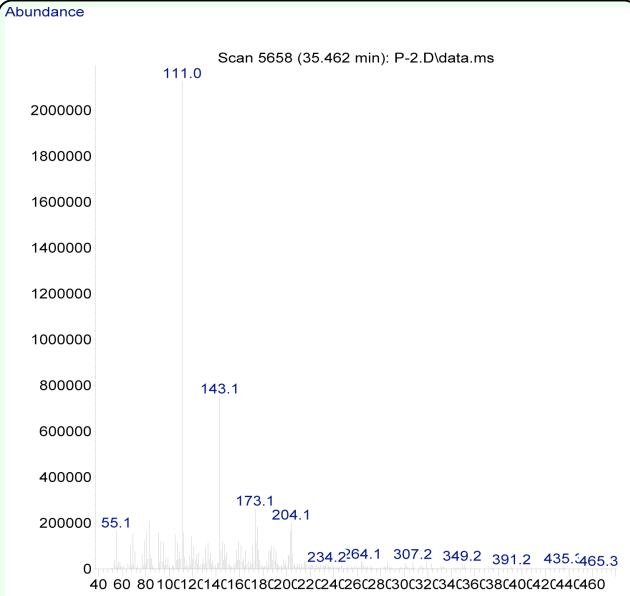
Figure 6. Mass spectra of 15-methoxy-I4, 15-dihydroclerodin. High quality figures are available online.
