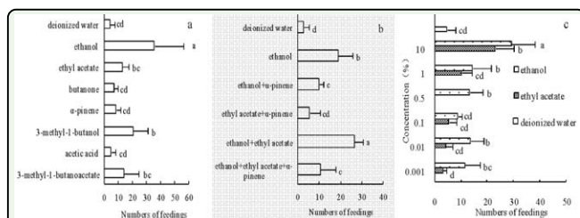
Figure 3. The feeding responses of Kallima inachus to different volatiles. A: single compounds at concentrations of 5%. B: compound mixtures at a total concentration of 5%. C: different doses of ethanol and ethyl acetate (mean \pm SD). Different letters indicate significant differences with the LSD test ( p < 0.05 ). High quality figures are available online.
