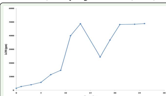
Figure 1. Resistance development of NJ-R Bemisia tabaci strain selected with chlorpyrifos in a dose of around LC_{70} in laboratory. LC_{50} s were examined every two or three generations. The selection by chlorpyrifos was stopped from the 13 th to 16 th generation, and then restored at the 26 th generation. High quality figures are available online.
