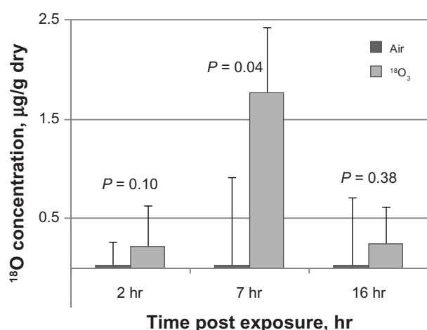
Figure 5. Concentration of excess ^{18}\text{O} in blood plasma from rats breathing 5 ppm ^{18}\text{O}_3 for 2 hours at 2, 7 and 16 hr post exposure. Significantly elevated plasma ^{18}\text{O} was observed at 7 hr post exposure.
