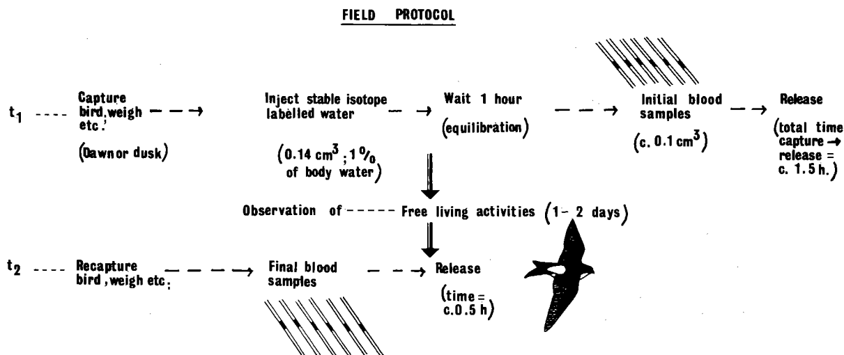
Fig. 1. Protocol for D_2O^{18} technique under field conditions. Stable isotopes were introduced by intraperitoneal injection (c. 0.14 cm^3 = 1 per cent of body water). The initial blood samples were taken 1 hour after injection and consisted of six capillaries, together containing c. 0.1 cm^3 blood. A similar volume of blood was collected after one or two days of free living activity. Further details of methods are given by Hails (1977) and by Hails & Bryant (1979).
