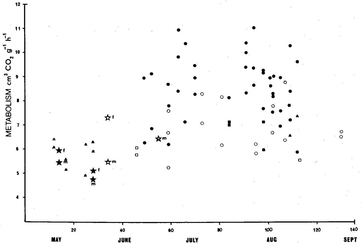
Fig. 4. Individual measurements of ADMR throughout the breeding season. Four breeding stages are distinguished: non breeding \triangle , laying \star (males, m; females, f), incubation \blacksquare and rearing \bullet . Open symbols 1977 data, closed symbols 1978 data. Metabolism plotted on data, where May 1 = 0.
