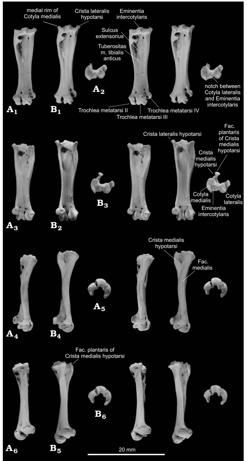
Fig. 1. Stereopairs of the holotypic left tarsometatarsus of miniature owl Glaucidium kurochkini sp. nov. (LACM RLB K9630), late Pleistocene, Rancho La Brea, California, USA (A) and a comparative left tarsometatarsus of Glaucidium californicum Sclater, 1857 (UCLA 38395), Recent, Western North America (B), in anterodorsal (A 1 , B 1 ), posteroventral (A 2 , B 2 ), medial (A 3 , B 3 ), lateral (A 4 , B 4 ), proximal (A 5 , B 5 ), and distal (A 6 , B 6 ) views. Abbreviations: Fac., Facies; m., musculus.
