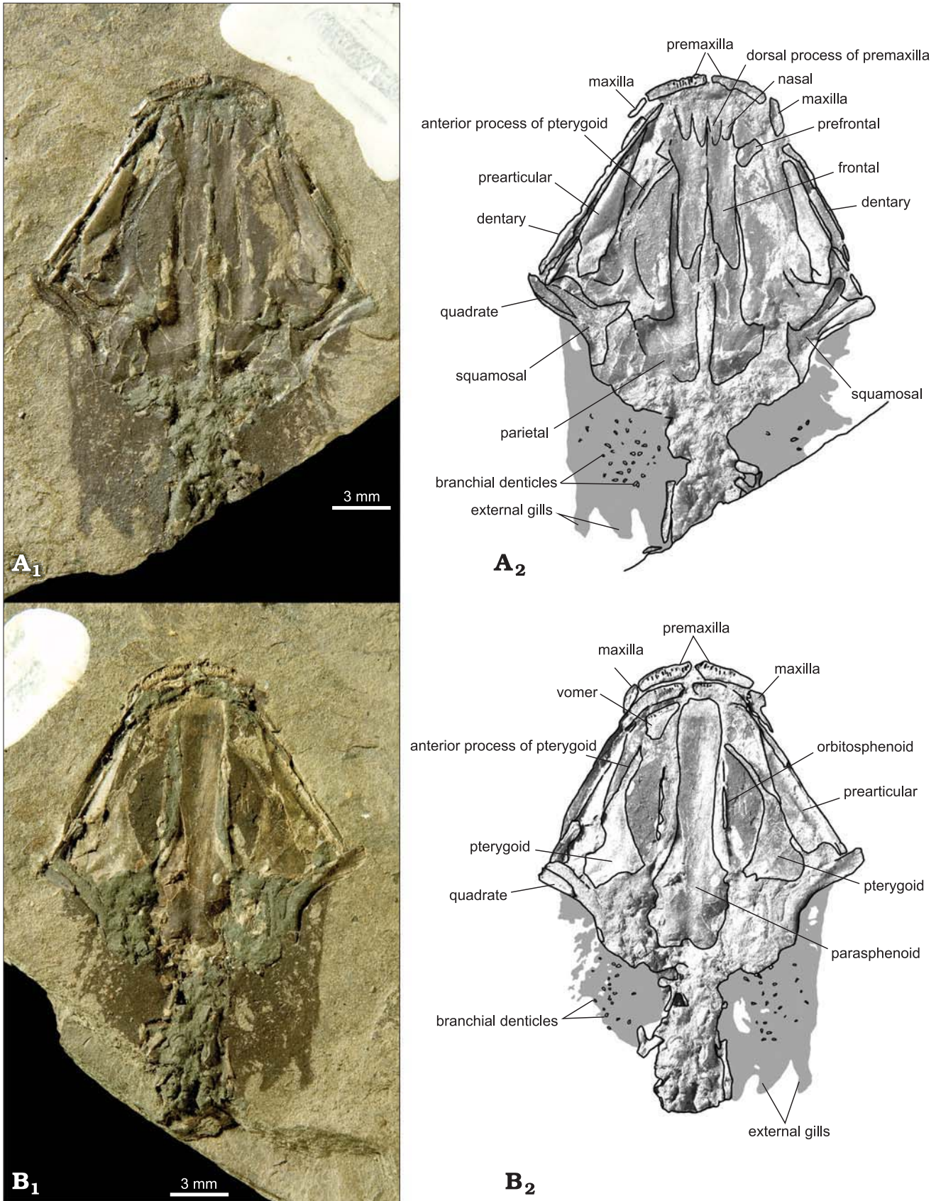
Fig. 1. A salamander Seminobatrachus boltischki gen. et sp. nov. from the lower unit of the Boltyszka sapropelite strata (late Paleocene–early Eocene, Ukraine), skull and anteriormost vertebrae with traces of soft tissue, holotype, PIN 3991/9. A. PIN 3991/9a, part in dorsal aspect. B. PIN 3991/9b, counterpart in ventral aspect. Photographs as exposed ( A 1 , B 1 ) and interpretative drawings ( A 2 , B 2 ). Grey areas in interpretive drawings represent soft tissues.
