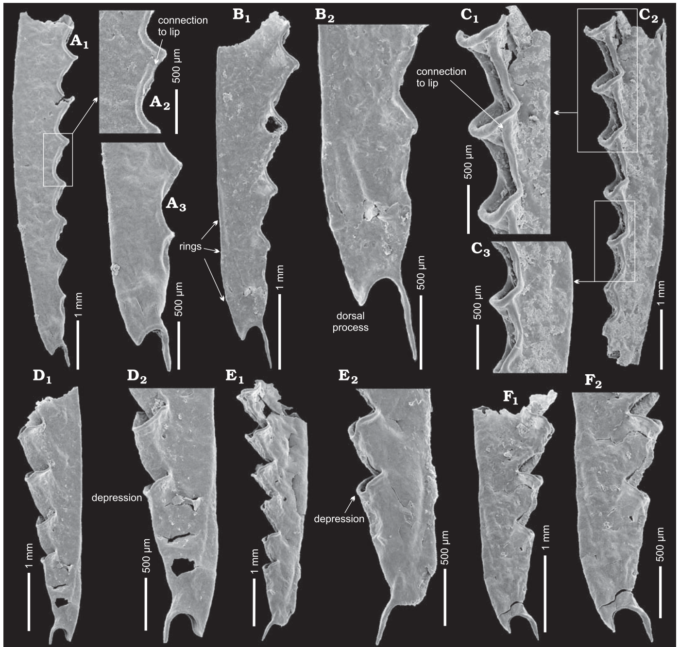
Fig. 13. SEM micrographs of Ludfordian graptolites Pristiograptus dubius postmagnus subsp. nov. and Pristiograptus dubius labiatus Urbaneck, 1997. A–C. Pristiograptus dubius postmagnus subsp. nov., Mielnik-1 borehole, Poland, depth 780.5 m; Monograptus (Uncinatograptus) acer Biozone. A. ZPAL G.44/48, lateral view of rhabdosome (A 1 ), thecal lip with connection to the succeeding theca (A 2 ), and proximal end of rhabdosome (A 3 ). B. ZPAL G.44/49, lateral view of rhabdosome sicula with rings (B 1 ) and proximal end of rhabdosome (B 2 ). C. ZPAL G.44/50, medial part of rhabdosome (C 2 ), enlargements showing connections to the succeeding thecae (C 1 , C 3 ). D–F. Pristiograptus dubius labiatus Urbaneck, 1997, Mielnik-1 borehole, Poland, depth 753.3 m; Monograptus (Uncinatograptus) spineus–Neocolonograptus parultimus Interzone. D. ZPAL G.44/51, general view of rhabdosome (D 1 ), sicula with two first thecae and depression on th 1 lip (D 2 ). E. ZPAL G.44/52, lateral view of rhabdosome (E 1 ) and proximal end of rhabdosome (E 2 ). F. ZPAL G.44/53, lateral view of rhabdosome (F 1 ) enlargement of proximal end (F 2 ).
