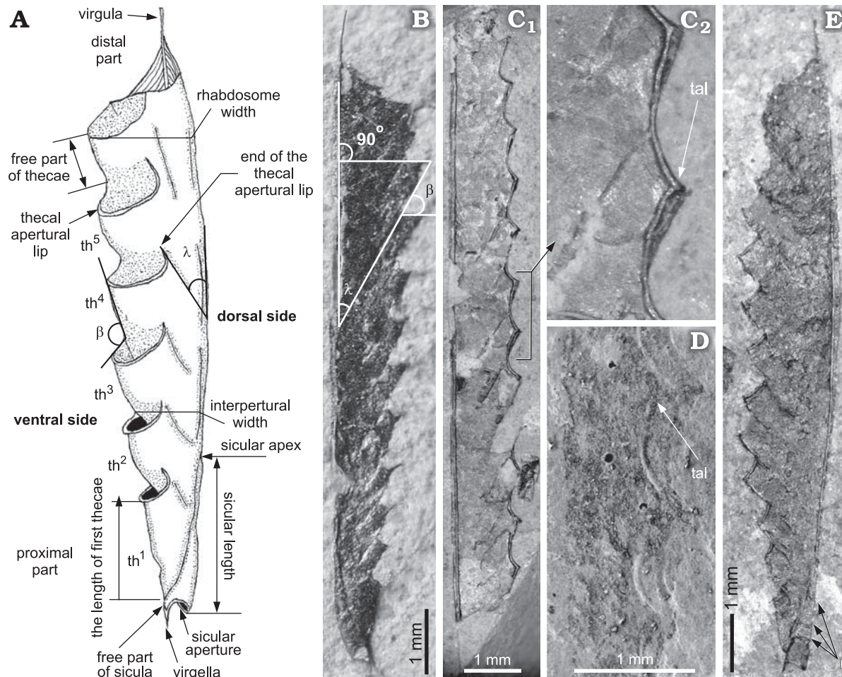
Fig. 3. Morphology of graptolite Pristiograptus rhabdosomes. A . Drawing of rhabdosome showing its characters (modified from Radzevičius 2003). B–E . Morphological features on flattened specimens. B . Pristiograptus lodenicensis Příbyl, 1948; VU-813, Likėnai-396 borehole, Lithuania, depth 589.5 m; Cyrtograptus lundgreni Biozone, Riga Formation. C . Pristiograptus dubius magnus subsp. nov., VU-835, Parovėja-9 borehole, Lithuania, depth 599.8 m; Cyrtograptus perneri Biozone, whole specimen (C 1 ), enlargement showing thecal apertural lip (C 2 ). D . Pristiograptus dubius pseudodubius (Bouček, 1932), fragment of rhabdosome, VU-A3-0047a; C. lundgreni Biozone, Źdanów outcrop, Sudetes, Poland. E . Pristiograptus jaegeri Holland, Rickards, and Warren, 1969; Vilkaviškis-131 borehole, depth 1073.2 m, VU-8004, Colonograptus deubeli Biozone. Abbreviations: \beta , angle between thecal lip and wall of succeeding theca; \lambda , angle between interthecal septum (thecal axis) and virgule; r, sicular ring; th 1 , first theca; tal, thecal apertural lip.
