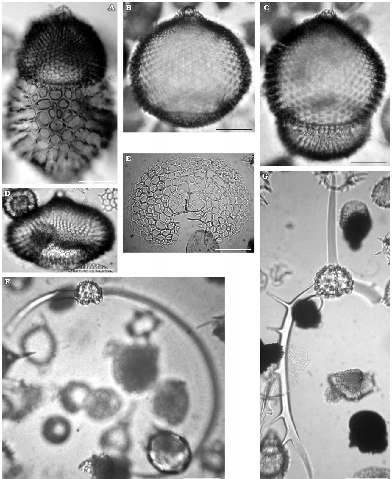
Fig. 13. Radiolarians from the early Miocene to Pleistocene of the eastern equatorial Pacific. A. Lophocyrtis (Cyclampterium) leptetrum (Sanfilippo and Riedel, 1970). MPC-3322; 845A-24XCC, R43/3; Zone RN5. B. Lophocyrtis (Cyclampterium) neatum (Sanfilippo and Riedel, 1970). MPC-4847; 1241A-29H-03, 62–64 cm, O14/0; Zone RN7. C. Lophocyrtis (Cyclampterium) tanythorax (Sanfilippo and Riedel, 1970). MPC-4854; 1241A-31H-03, 62–64 cm, L40/0; Zone RN7. D. Lophocyrtis (Cyclampterium) brachythorax (Sanfilippo and Riedel, 1970). MPC-4870; 1241A-36X-03, 62–64 cm, S32/3; Zone RN6. E. Nephrospyris renilla Haeckel, 1887. MPC-3337; 1241A-3H-04, 75–77 cm, T37/0; Zone RN14. F. Dorcadospyris alata (Riedel, 1959). MPC-3322; 845A-24XCC, R45/0; Zone RN5. G. Dorcadospyris dentata Haeckel, 1887. MPC-3328; 845A-30XCC, G39/0; Zone RN4. Scale bars 100 \mu m.
